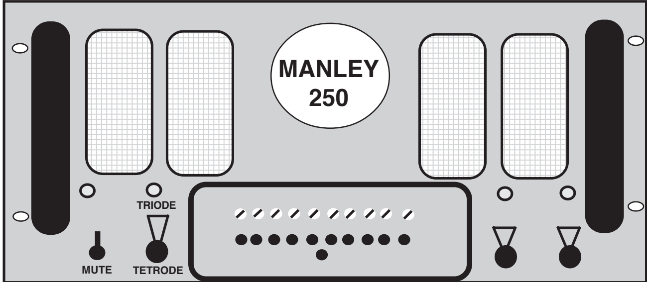
1 2 3 4 5 6 7 8 9 10 GROUND FRONT VIEW OF AMPLIFIER WITH INSERT REMOVED OPERATE STANDBY EVER-WARM SOFT START SWITCH MAINS POWER ON / OFF SWITCH SHOWING BIAS MEASUREMENT POINTS AND BIAS ADJUST POINTS
