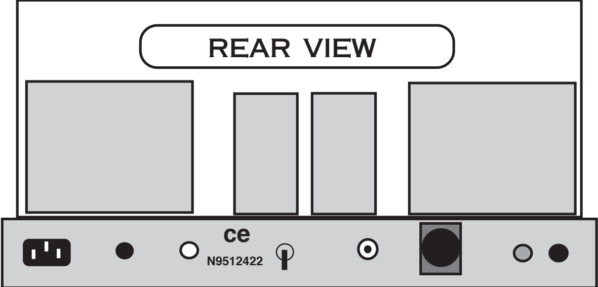
ce N9512422 MAINS IN IEC MAINS FUSE SLO-BLO B+ FUSE SLO-BLO BALANCED UNBALANCED SWITCH RCA INPUT XLR BALANCED INPUT SPEAKER OUTPUT BINDING POSTS
